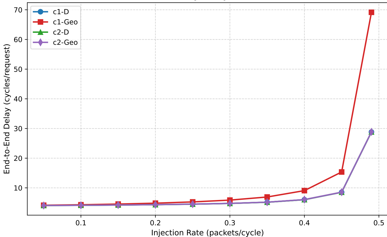
E2: end-to-end delay vs injection rate (B = 1)
