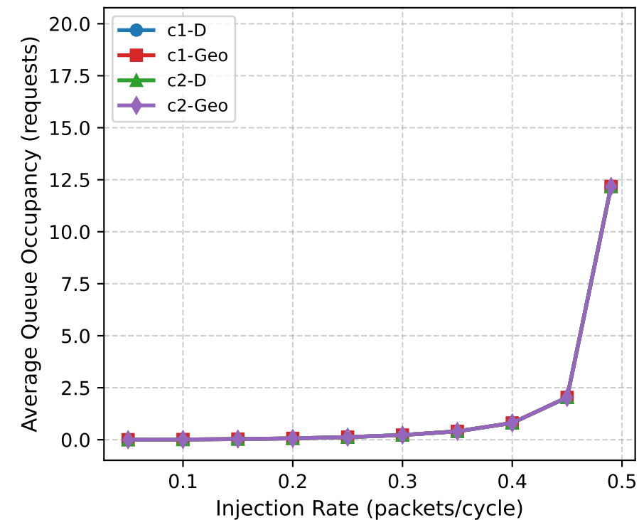
Q1 admission (Geo/D/1)
