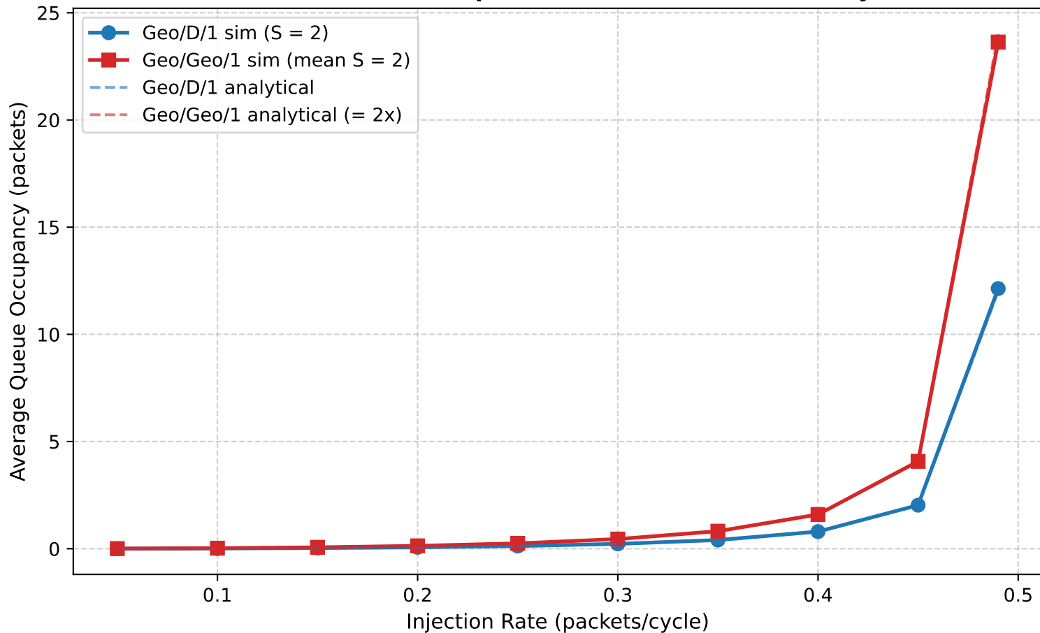
V2: factor-2 relationship, Geo/D/1 vs Geo/Geo/1 ( 10^7 cycles)
