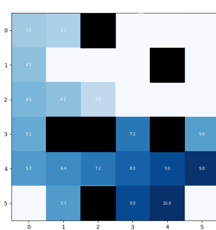
Figure 3: Q-Value Heatmap
