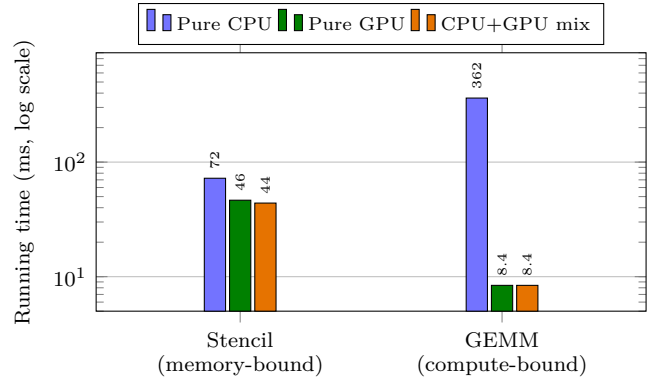
Fig. 1. Pure CPU vs. pure GPU vs. optimal CPU+GPU mix (lower is better, log scale). The mix wins outright on the memory-bound stencil (43.9 ms, 1.65\times over CPU, 1.06\times over GPU); on the compute-bound GEMM the GPU is 43\times the CPU, so the predicted split sends 97.7% to the GPU and the mix matches pure GPU (8.4 ms).
