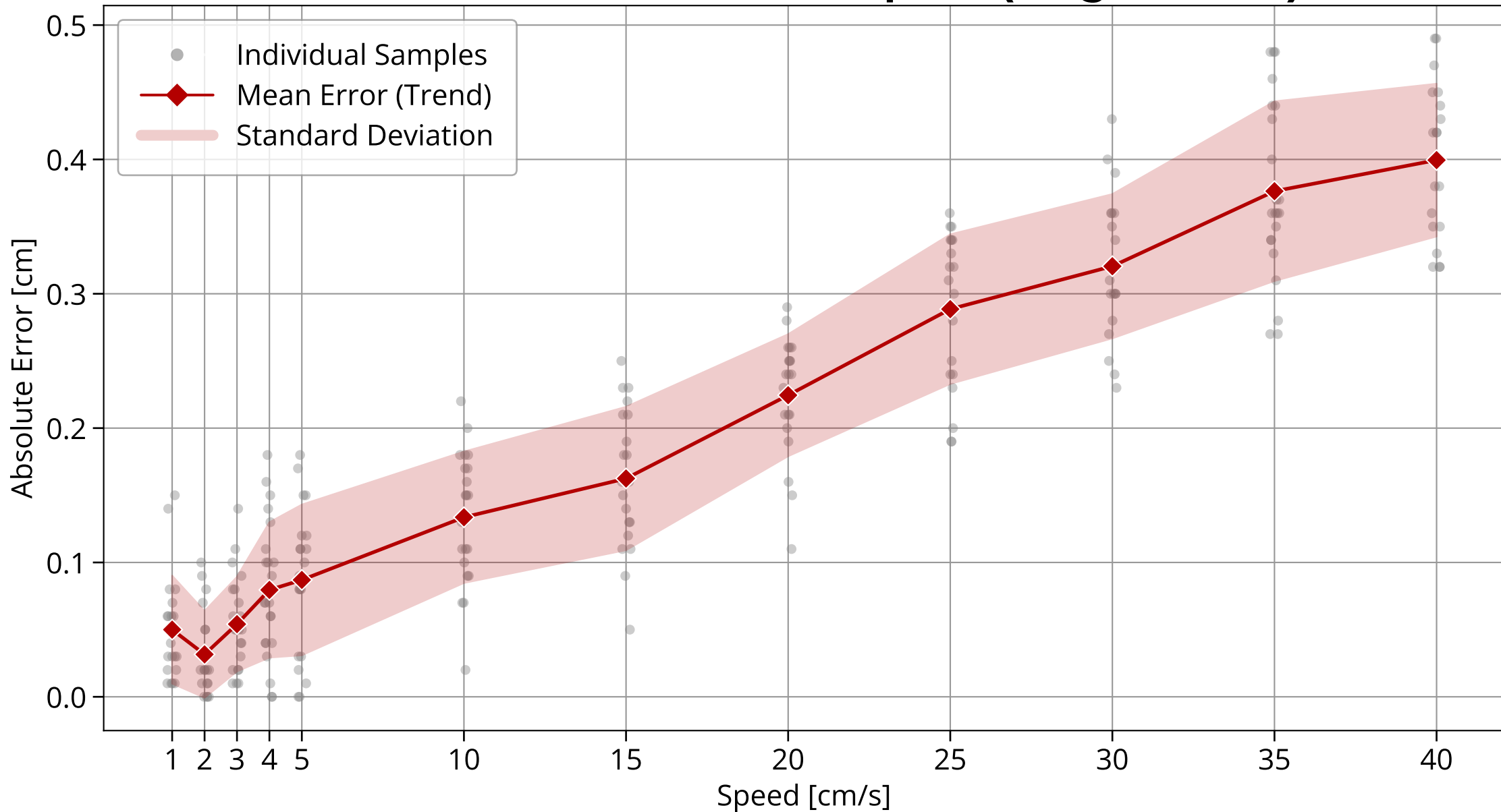
Encoder Absolute Error vs Speed (Target: 50cm)
