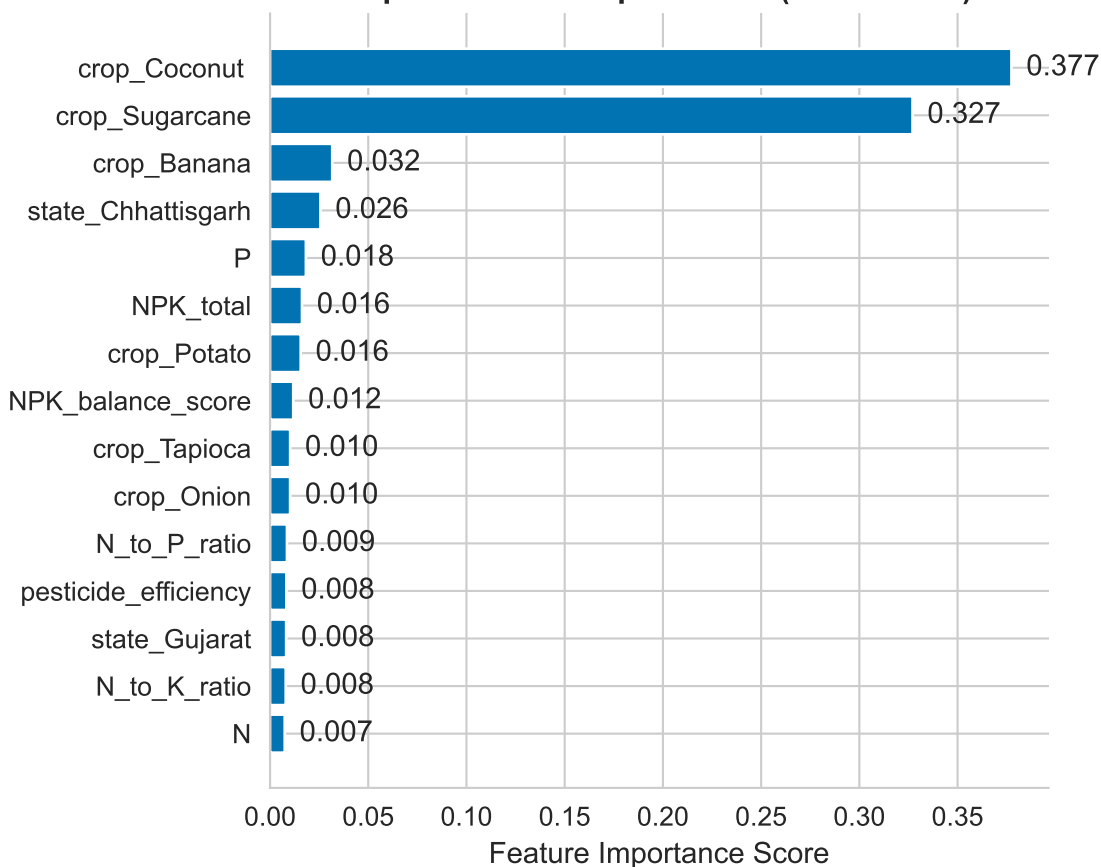
Top 15 Feature Importances (Extra Trees)
