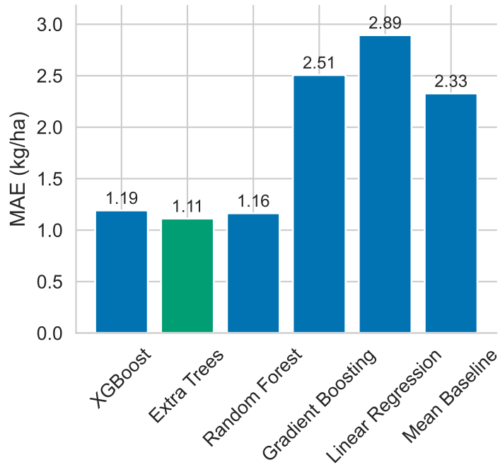
MAE Comparison
