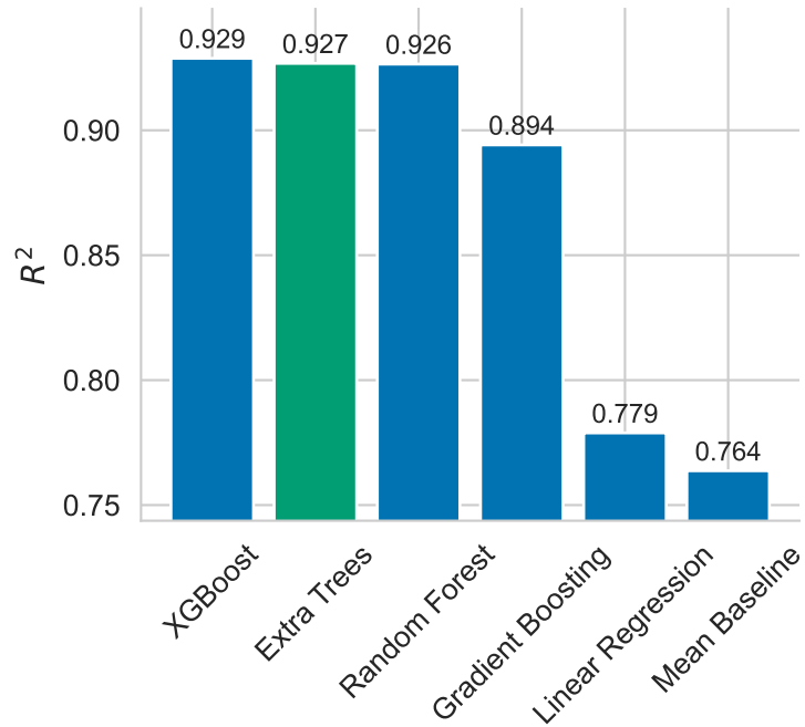
R^2 Comparison
