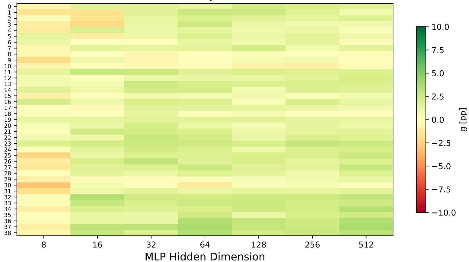
Accuracy Gain
