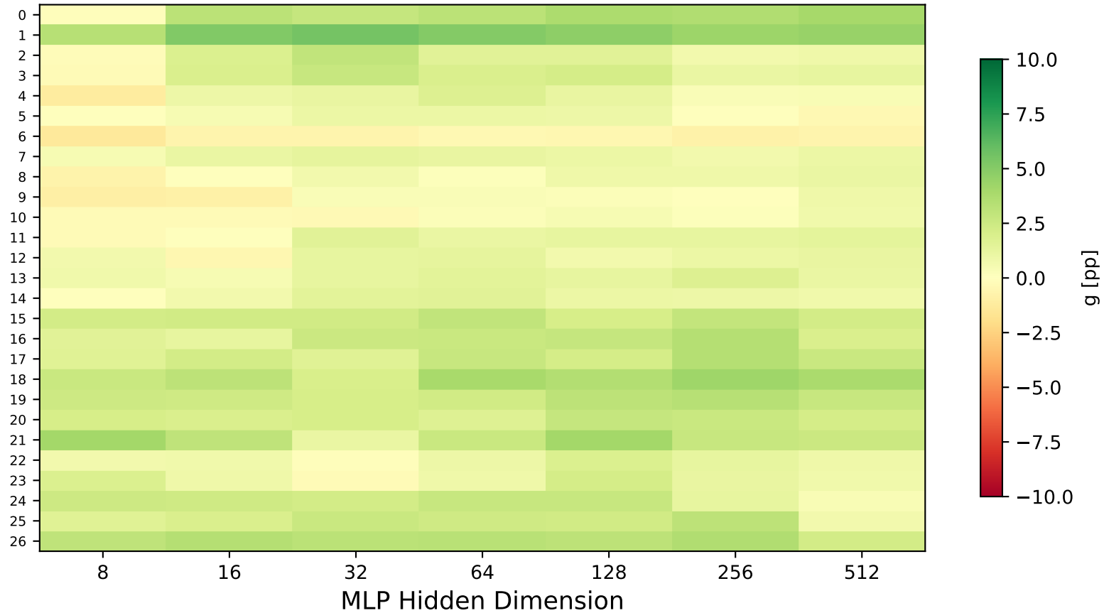
Accuracy Gain
