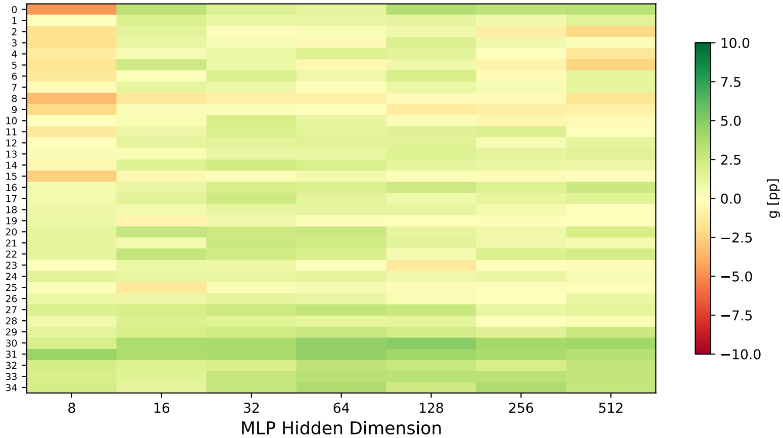
Accuracy Gain
