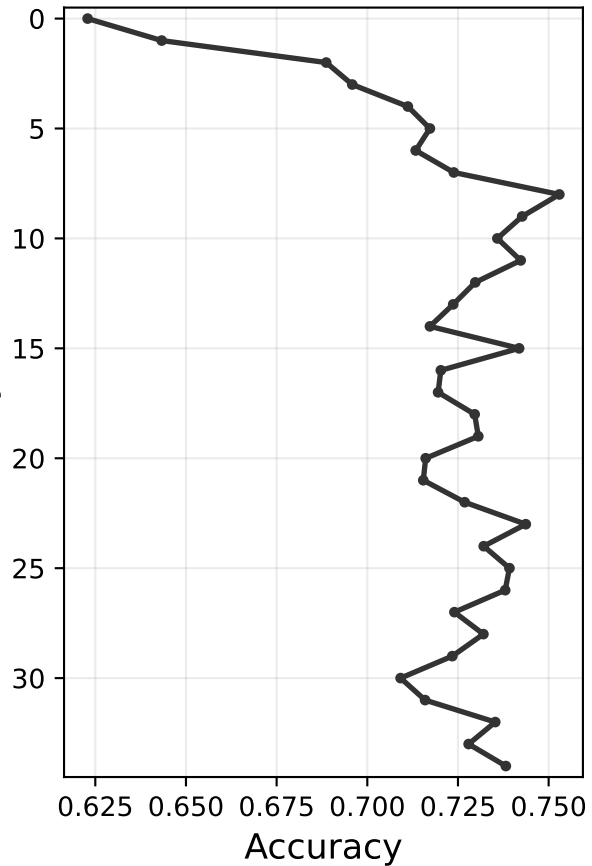
LR Baseline
