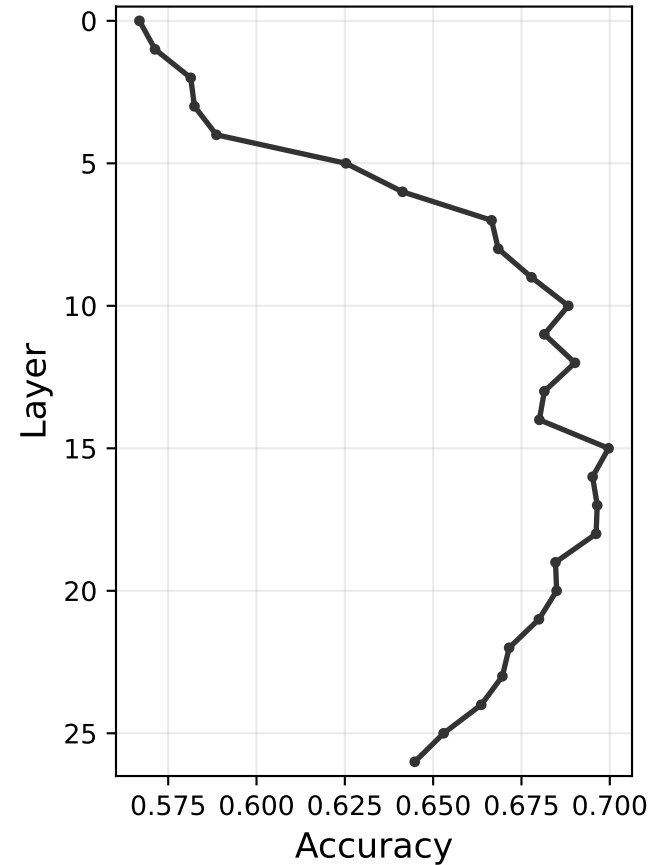
LR Baseline
