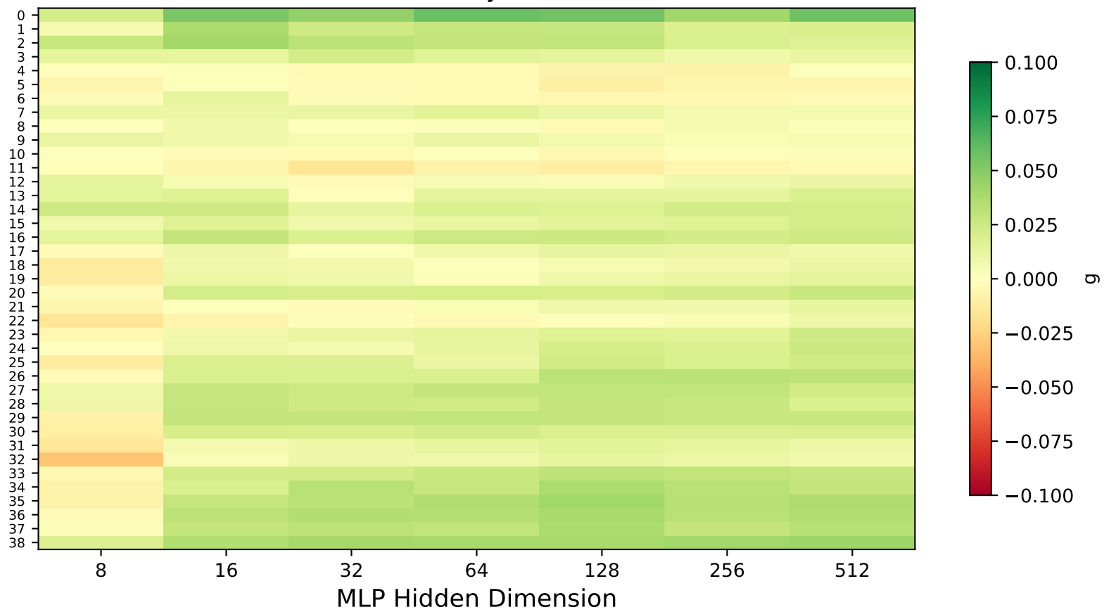
Accuracy Gain
