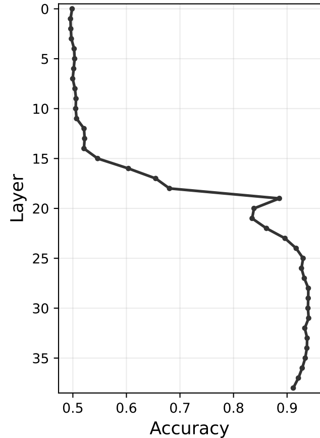
LR Baseline
