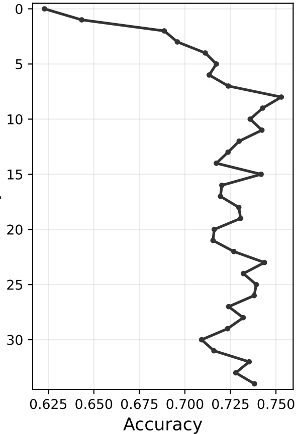
LR Baseline
