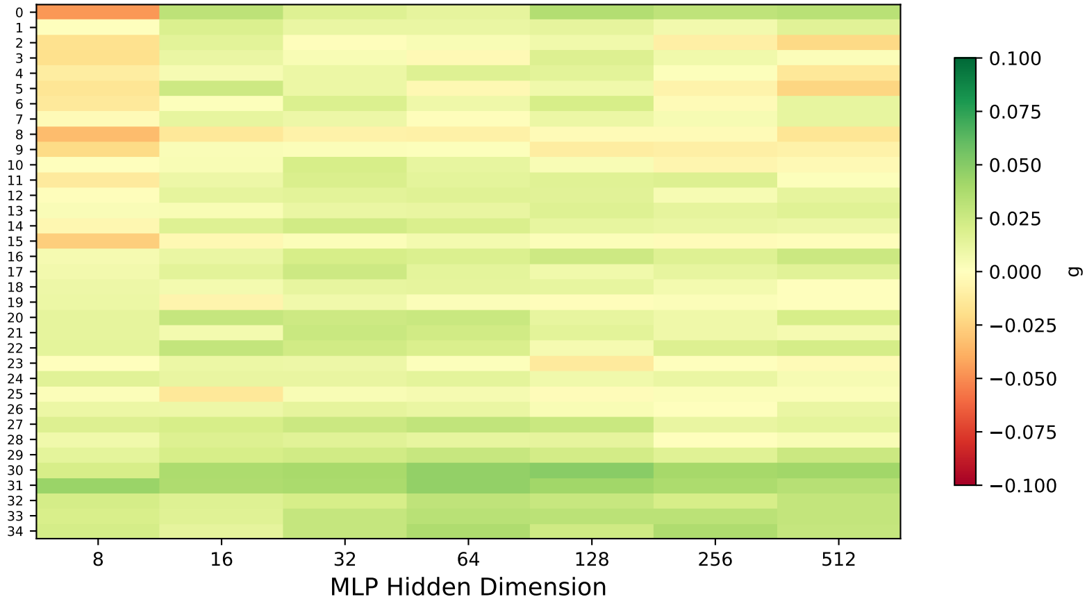
Accuracy Gain
