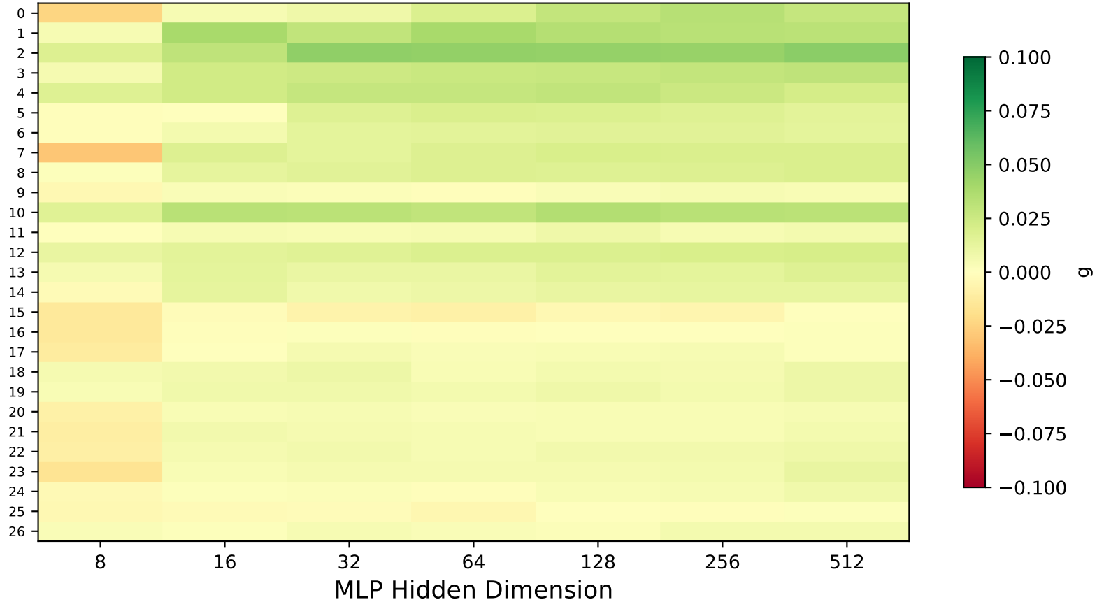
Accuracy Gain
