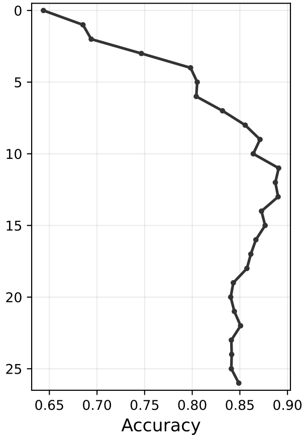
LR Baseline
