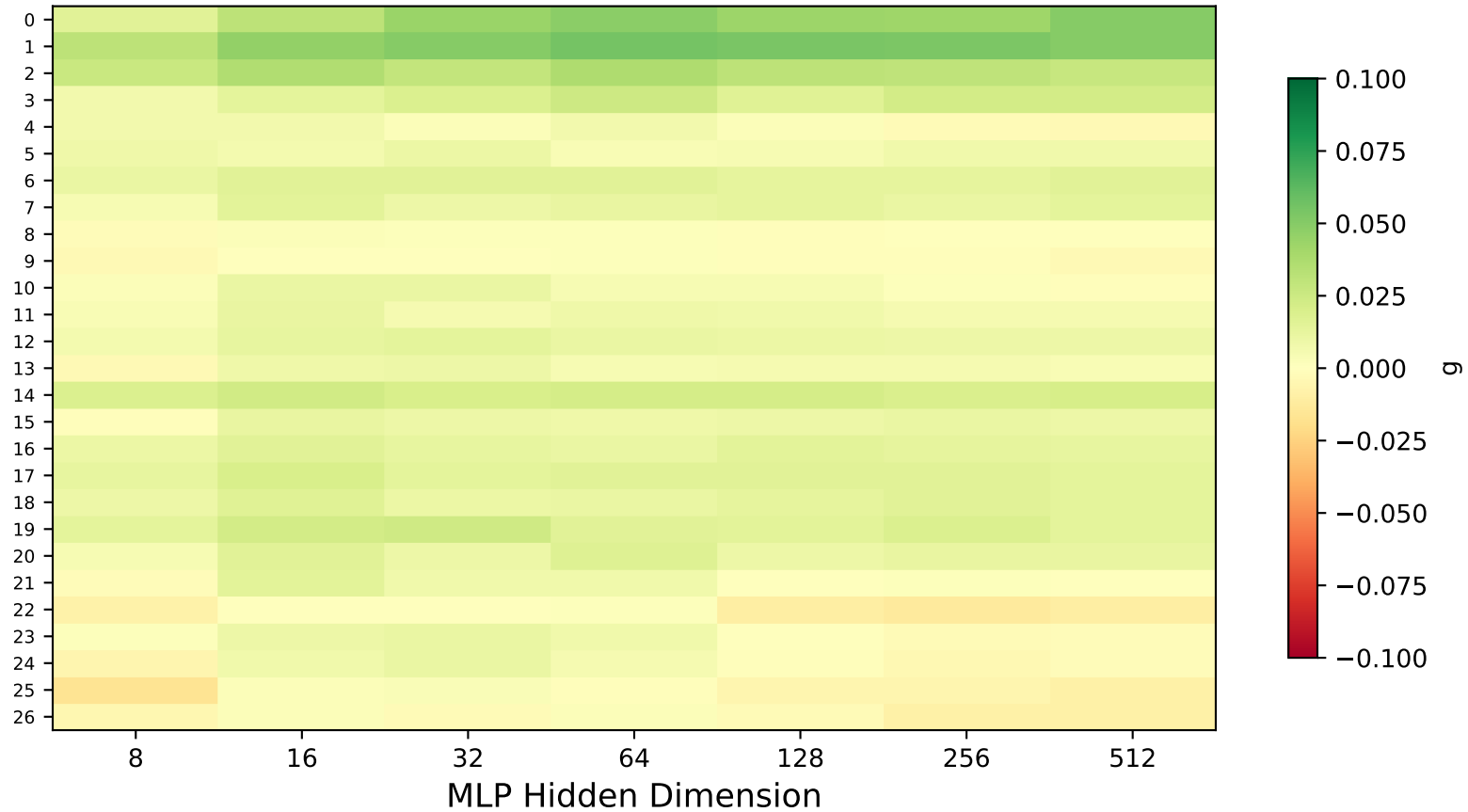
Accuracy Gain
