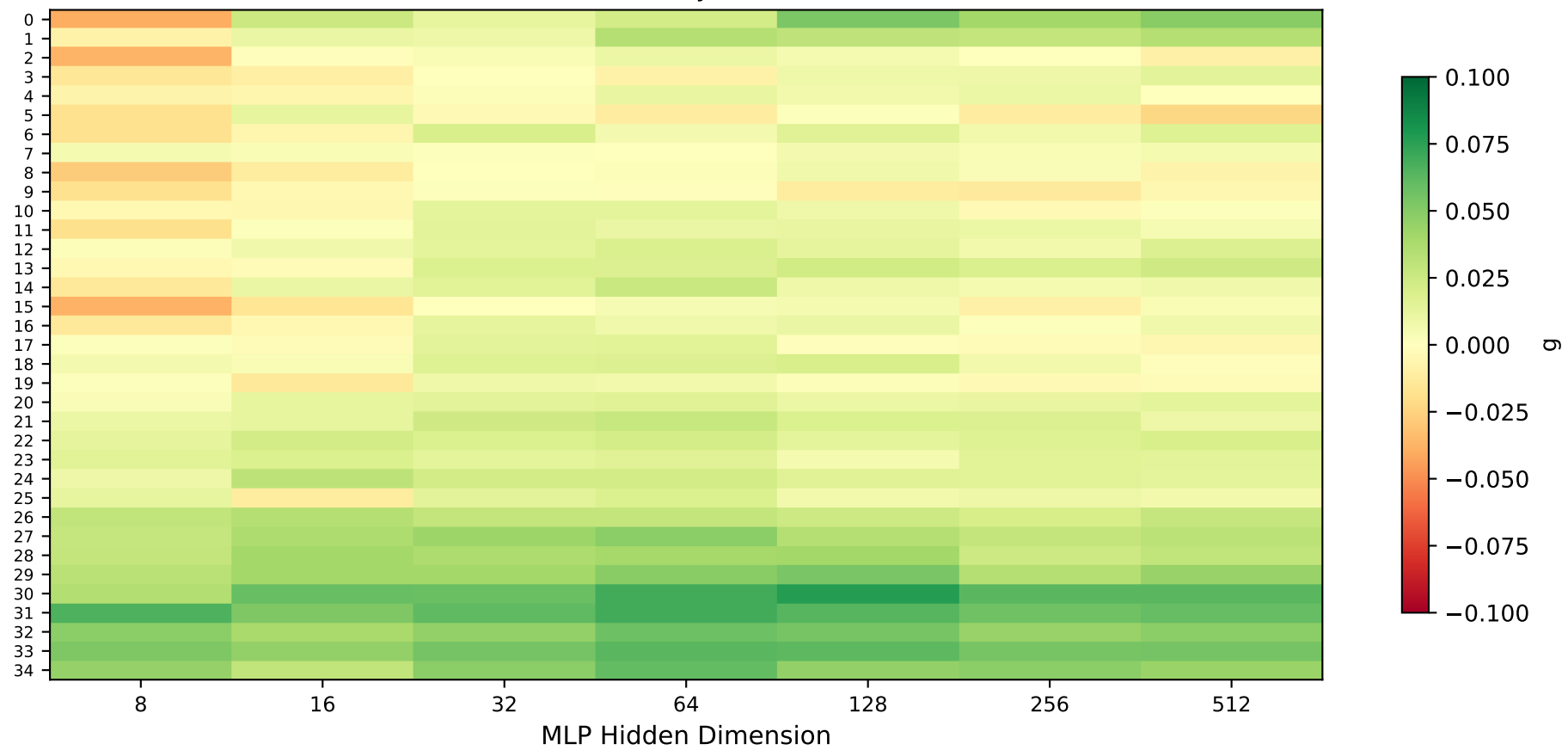
Accuracy Gain
