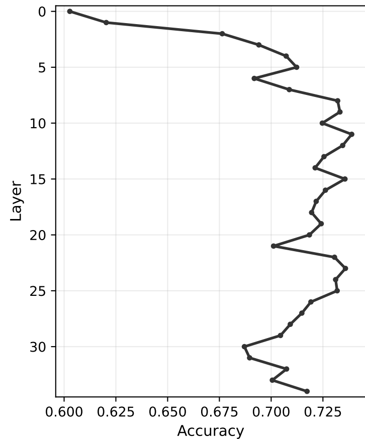
LR Baseline
