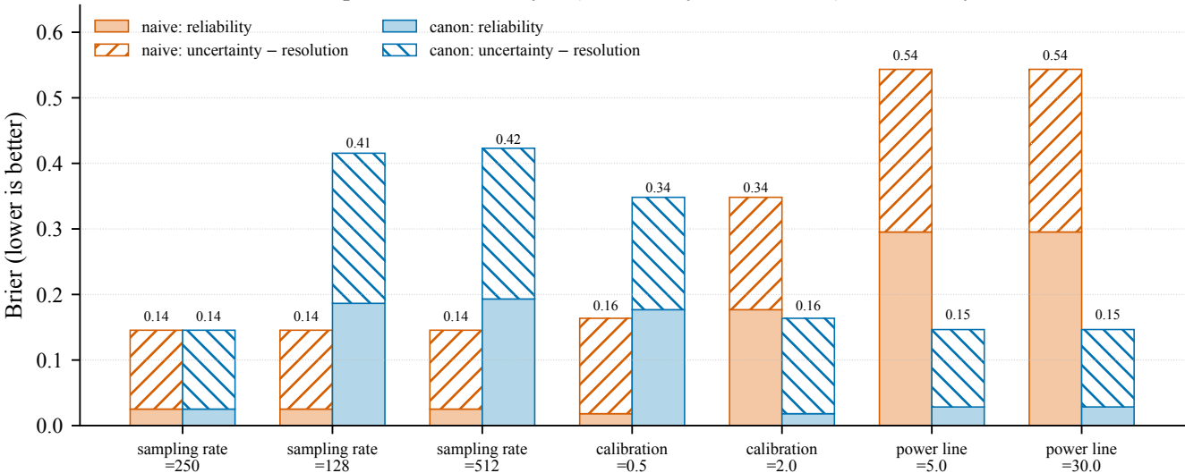
Brier decomposition: reliability + (uncertainty – resolution); uncertainty=0.248
