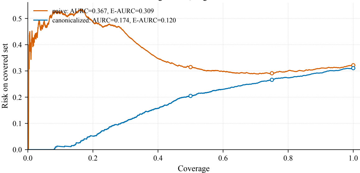
Risk-coverage curve, llogitl-rank abstention
