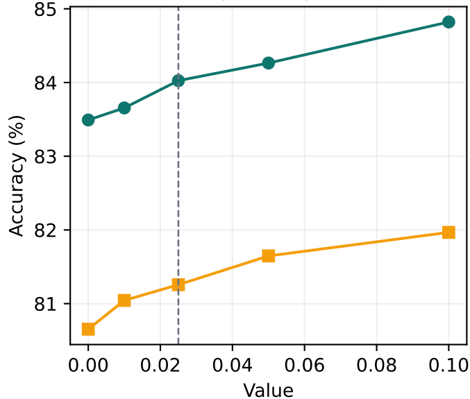
class prior strength
