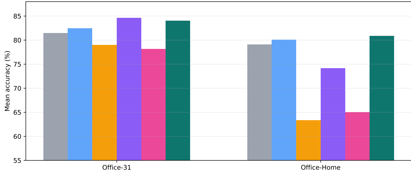
Mean accuracy under unified Office protocols
