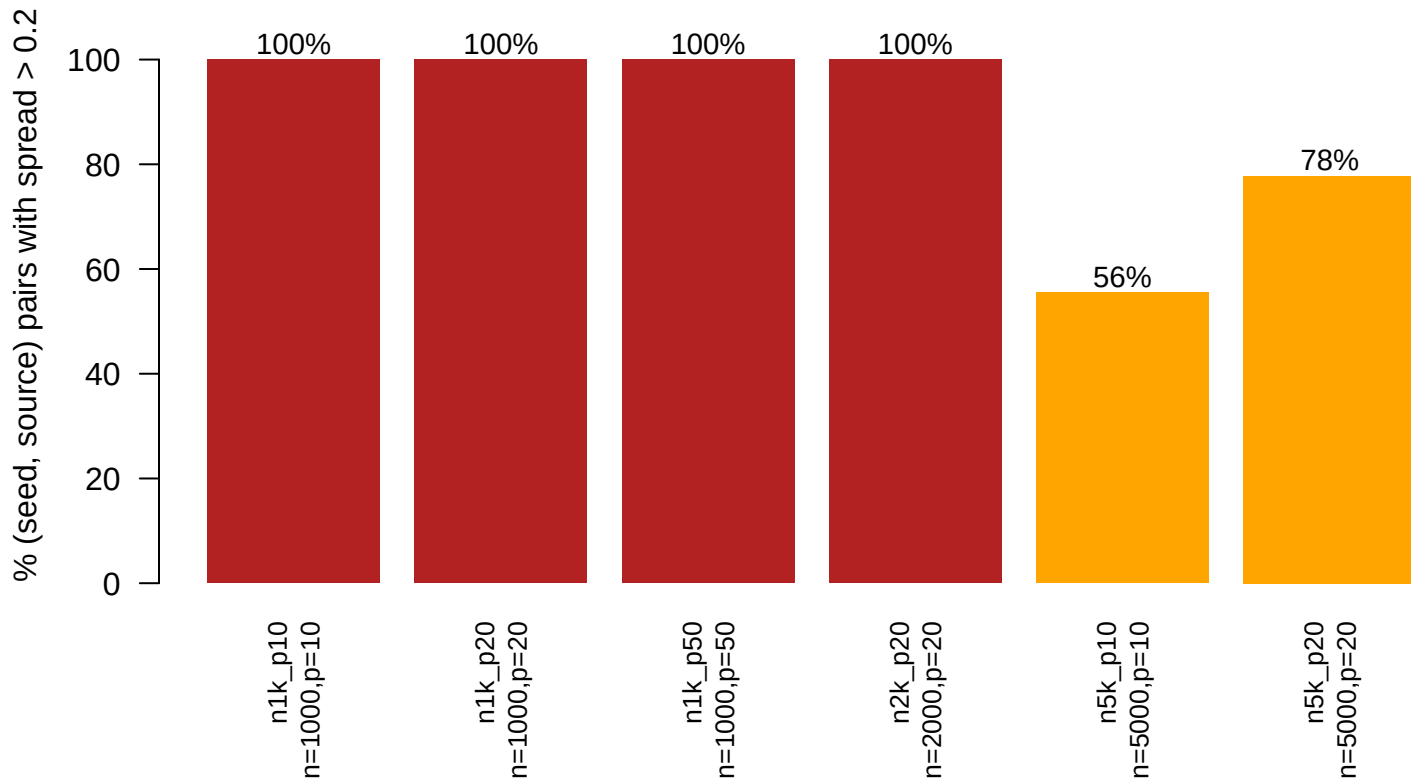
Explosion rate by (n, p) setting
