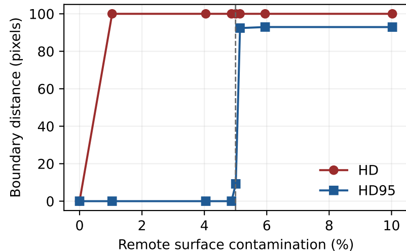
HD95 is robust below its 5% tail, then changes rapidly
