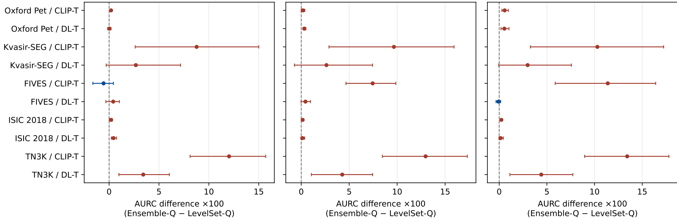
Dice risk
