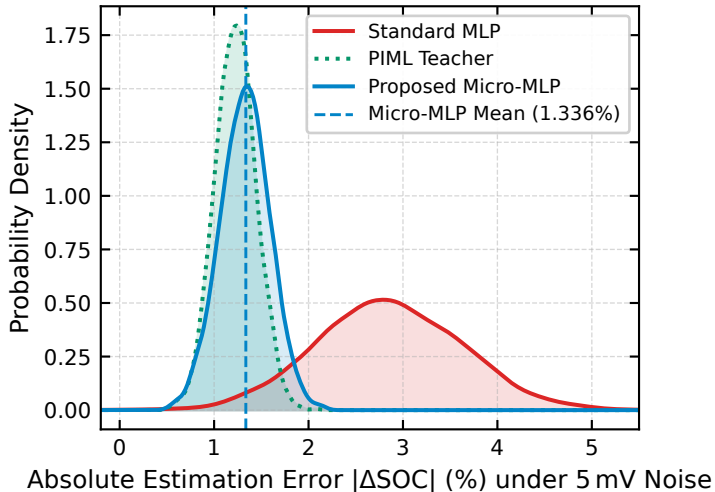
(b) Error Dispersion under 5.0 mV Noise
