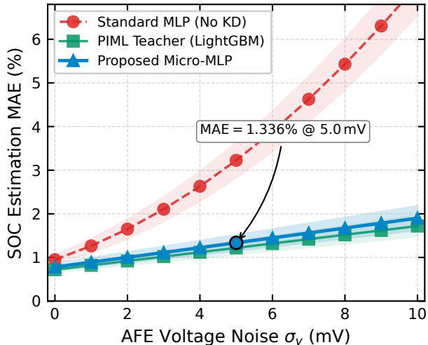
(a) Robustness vs. Sensor Noise Level
