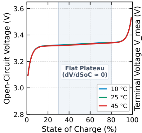
(a) LFP OCV-SoC Characteristic
