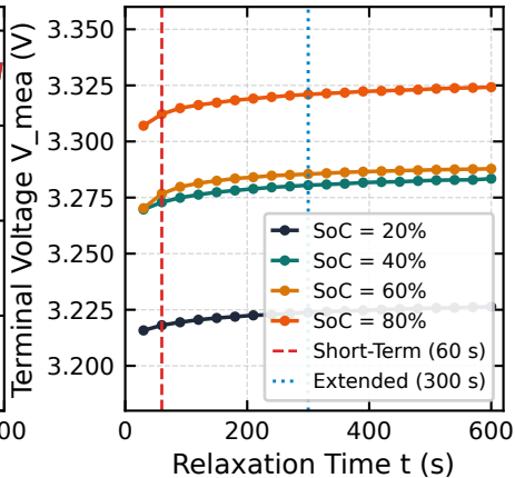
(b) Dynamic Relaxation Profiles
