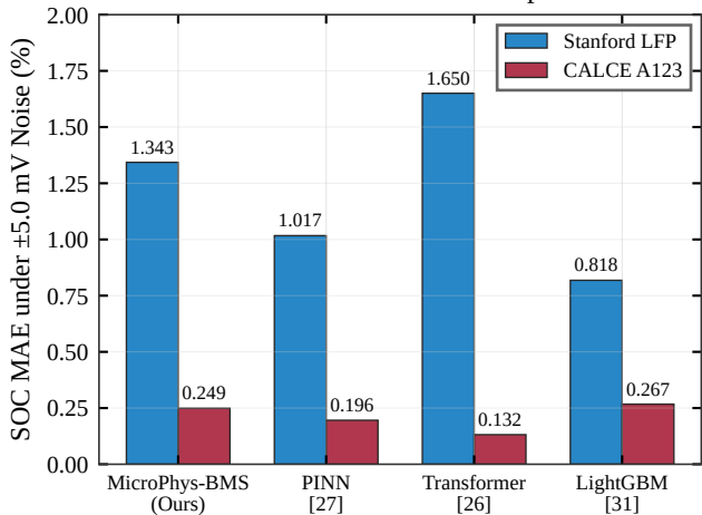
AFE Noise Robustness Comparison
