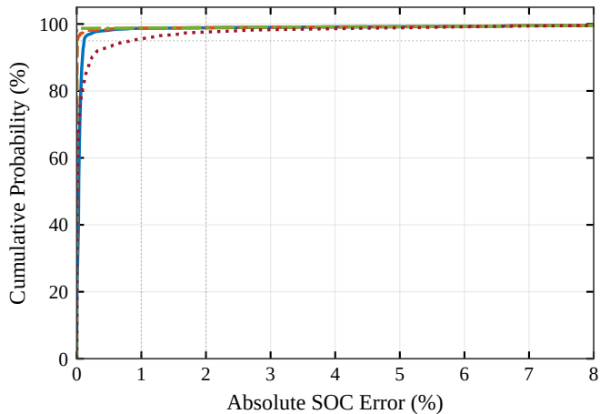
(b) CALCE A123 LFP (24 ° C)
