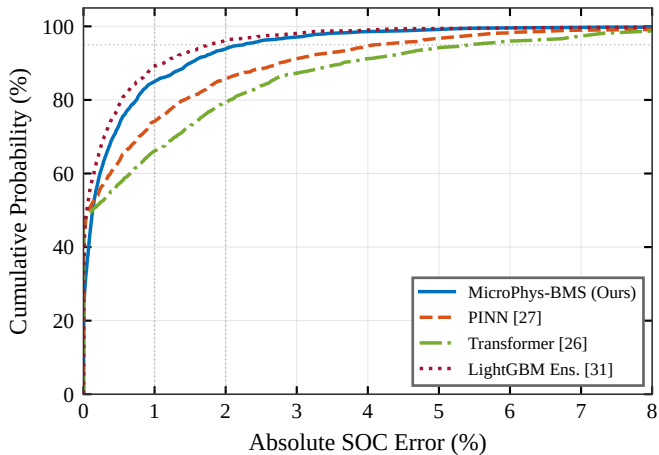
(a) Stanford LFP (25 ° C)
