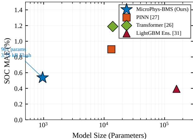
Accuracy-Complexity Trade-off
