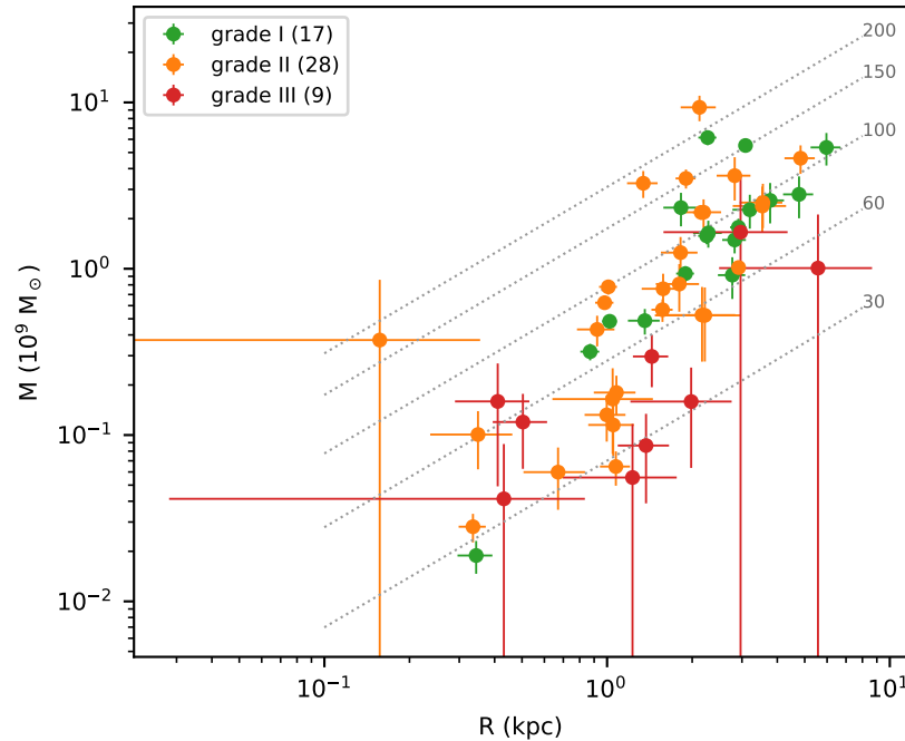
M-R plane; dotted: constant v_L (km/s)
