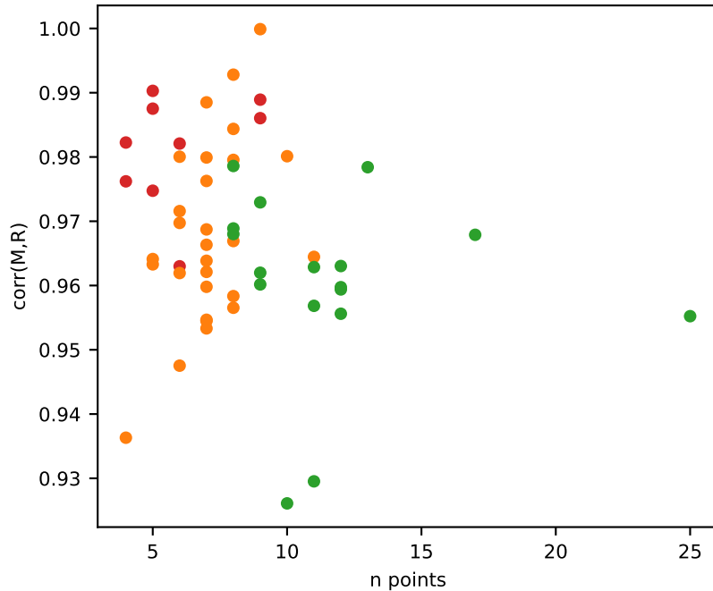
M-R degeneracy
