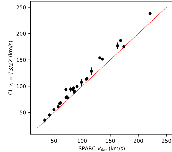
Asymptotic speed (28 with V_{flat} )
