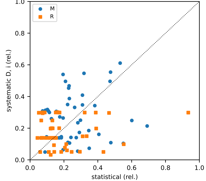
Stat. vs syst. uncertainty
