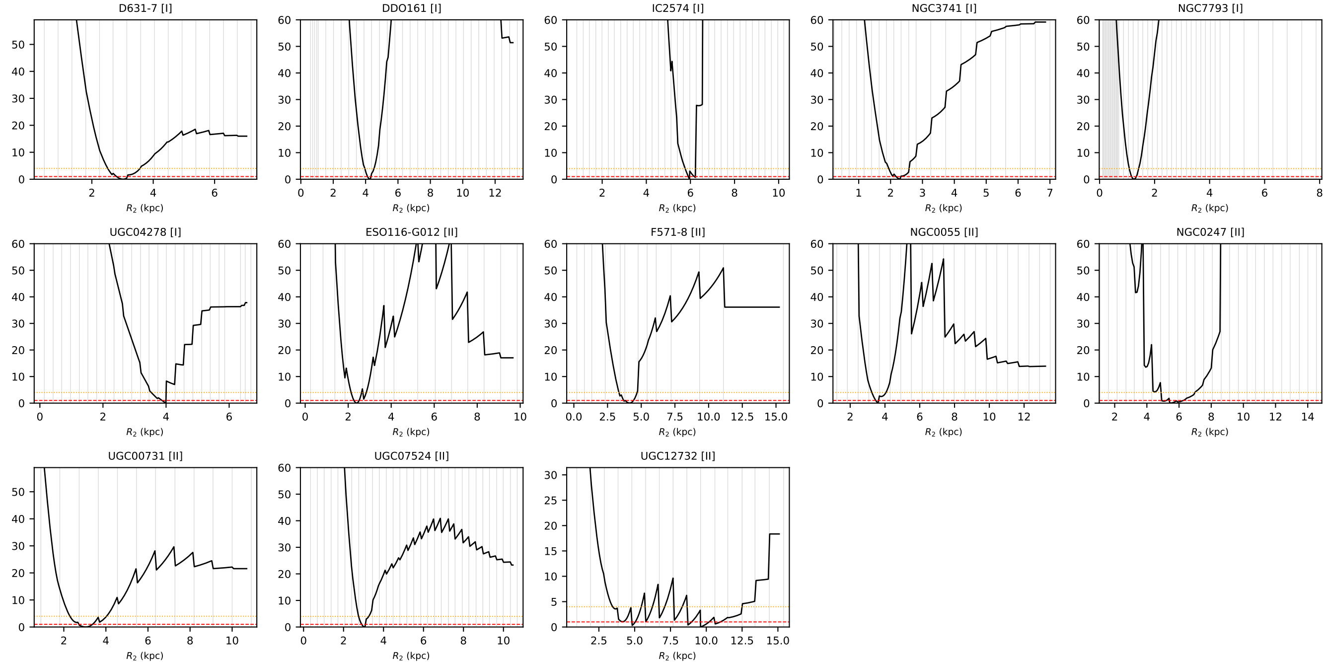
Profile \Delta\chi^2(R_2) for the clean nested galaxies (other parameters refitted); red: \Delta\chi^2 = 1 , orange: 4; grey: data radii
