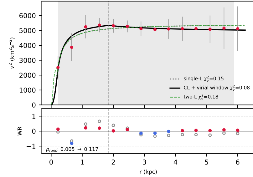
NGC1705 [single-L kept] n=14 r_v=1.9 , p=4.27 , \Delta\text{BIC}=4.3
