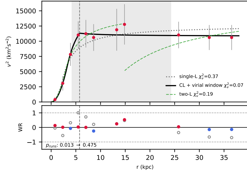
UGC01230 [single-L kept] n=11 r_v=5.8 , p=2.14 , \Delta\text{BIC}=1.9
