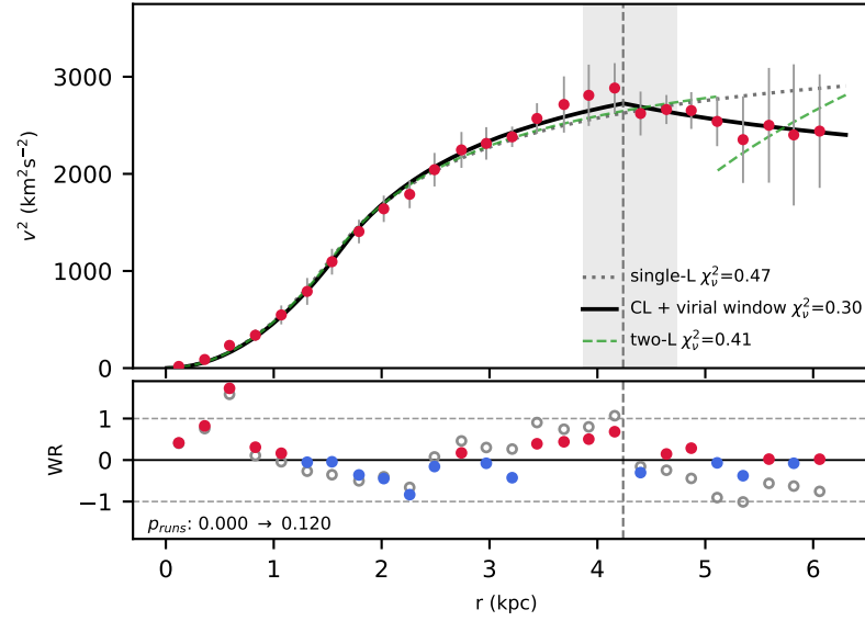
NGC2366 [single-L kept] n=26 r_v=4.2 , p=4.11 , \Delta\text{BIC}=1.9
