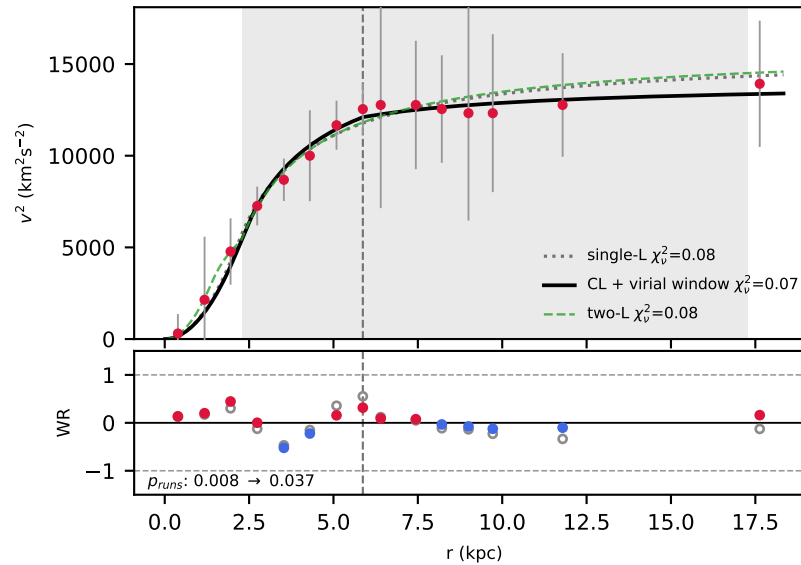
F568-V1 [single-L kept] n=15 r_v=5.9 , p=1.11 , \Delta\text{BIC}=5.1
