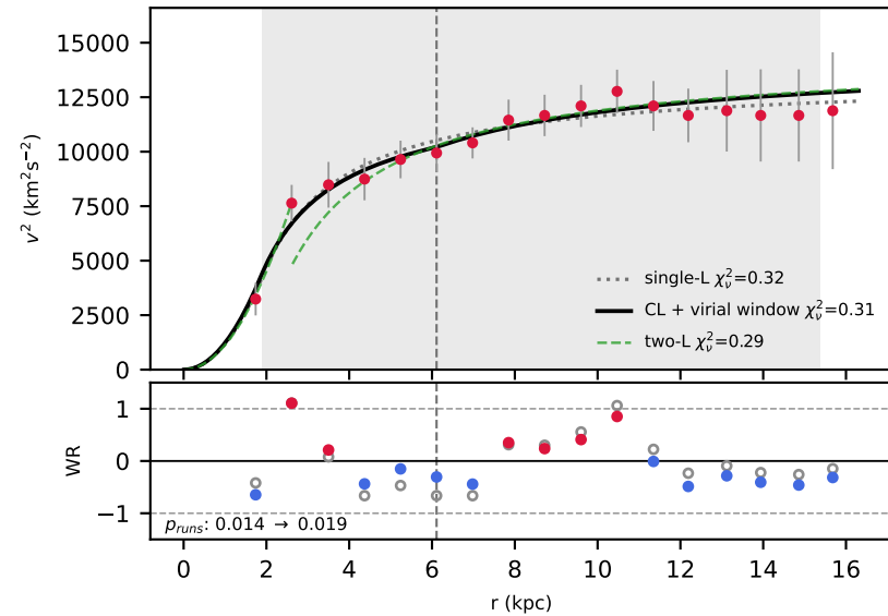
UGC06983 [single-L kept] n=17 r_v=6.1 , p=-1.13 , \Delta\text{BIC}=4.9
