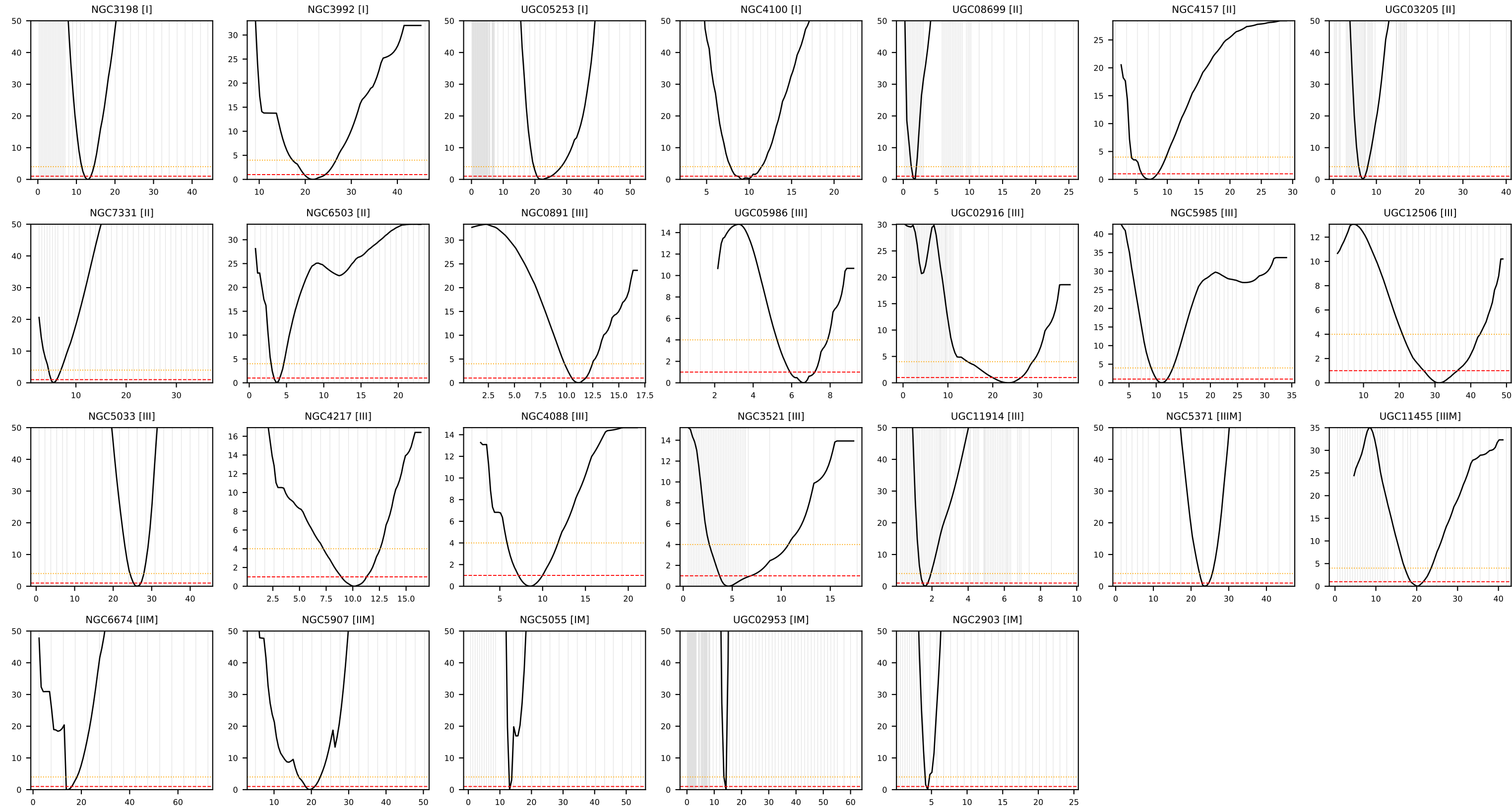
Profile \Delta\chi^2(r_v) for the descent-window galaxies (other parameters refitted); red \Delta\chi^2 = 1 , orange 4; grey: data radii
