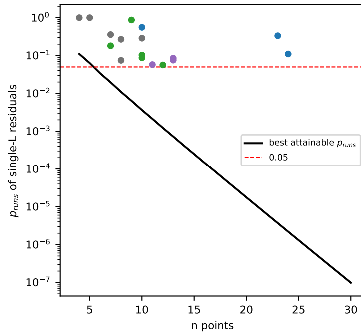
Power of the runs test
