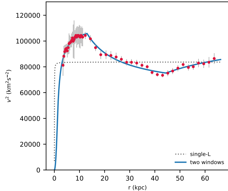
Multi-region NGC2841
