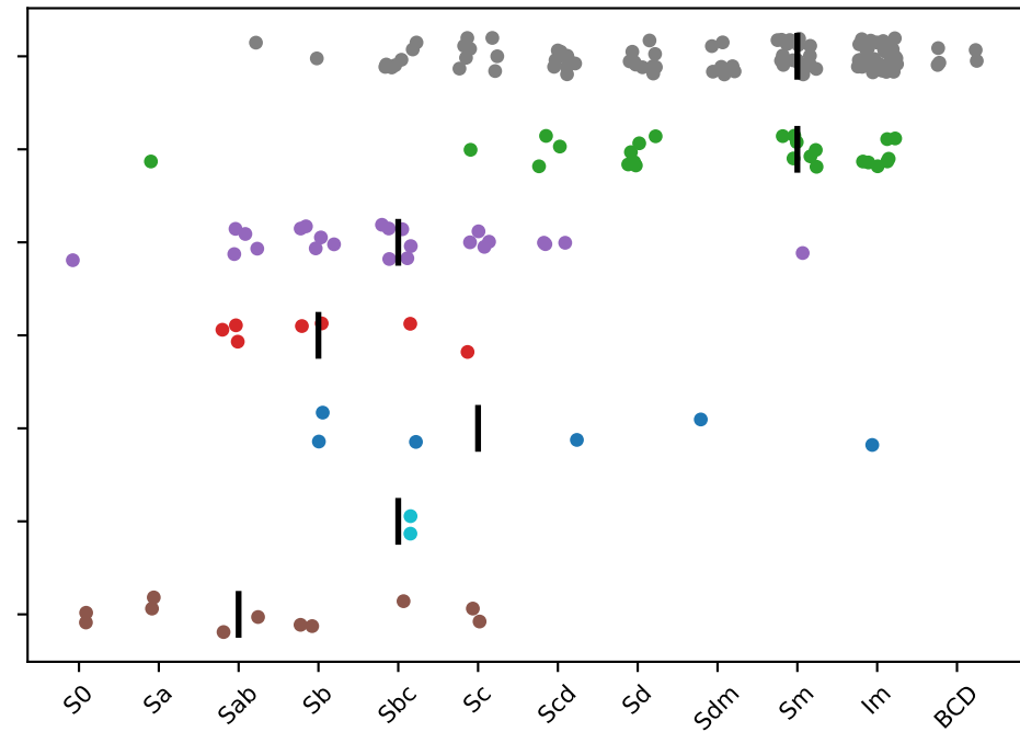
Hubble type per galaxy (bar: median)
