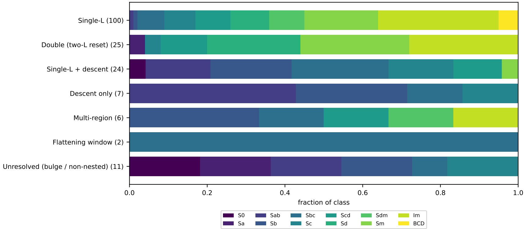
Hubble-type composition of each class
