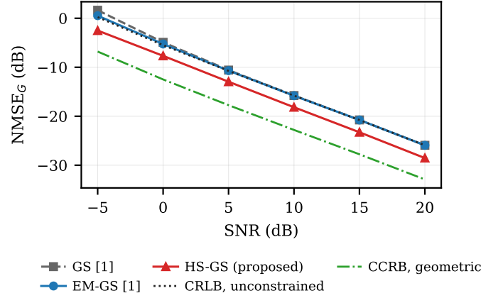
Fig. 1. NMSE versus SNR, bound-comparison configuration ( N = 32 , P = 30 , RSR 12 dB, T = 50 , 4 Cadzow sweeps, ratio-of-sums). EM-GS tracks the rank-one unconstrained CRLB closely at high SNR. Neither bound governs a biased estimator.
