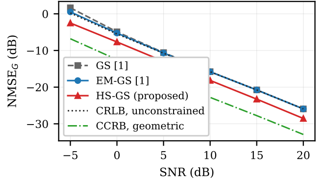
Fig. 1. NMSE versus SNR at N = 32 , P = 30 , \text{RSR} = 12 dB. EM-GS is indistinguishable from the unconstrained CRLB, so that bound is tight for the unstructured problem; HS-GS lies between the two, recovering part of the headroom identified by the geometric CCRB.
