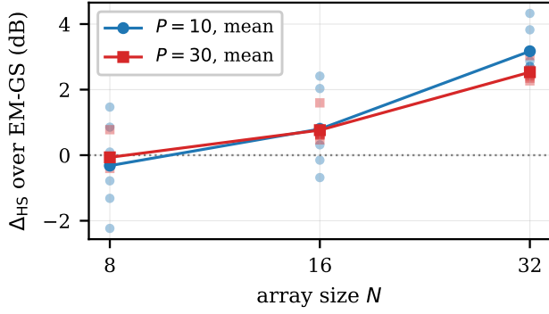
Fig. 2. Paired HS-GS gain over EM-GS versus array size. Faint markers are the six individual SNR operating points, solid lines their mean. The gain grows monotonically with N ; at N = 8 the points straddle zero, so no single scalar summarises that array size.
