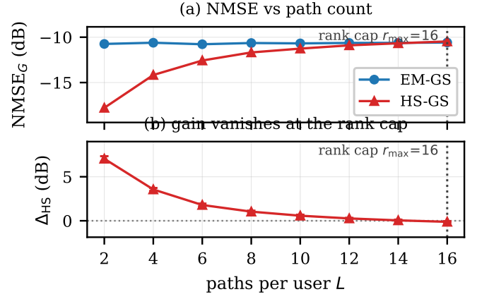
Fig. 3. Controlled path count ( N = 32 , P = 30 , \text{SNR} = 5 dB, \text{RSR} = 12 dB, 300 trials per point, L fixed and identical across users). (a) EM-GS is flat in L —path count does not affect an estimator that ignores structure—which confirms the sweep is not confounded; HS-GS rises to meet it. (b) The paired gain decays monotonically to zero as L approaches the rank ceiling r_{\max} = \lceil N/2 \rceil = 16 ; the 95% paired bootstrap band is plotted but is narrower than the markers. The hypothesis producing this figure was recorded before the experiment was run.
