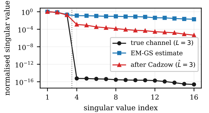
Fig. 4. Normalised Hankel singular values for one channel column, N = 32 , L = 3 , \text{SNR} = 5 dB. The true channel is exactly rank L , the EM-GS estimate is full rank, and Cadzow restores the cliff only approximately, to \sim 10^{-3} .
