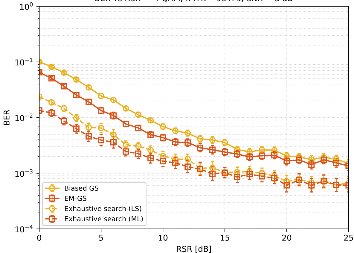
BER vs RSR — 4-QAM, N \times K = 36 \times 3 , SNR = 3 dB
