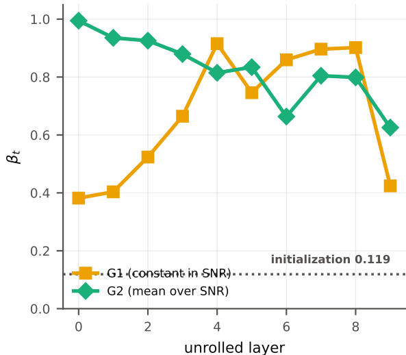
b. EARLY layers project hardest — I predicted the opposite
