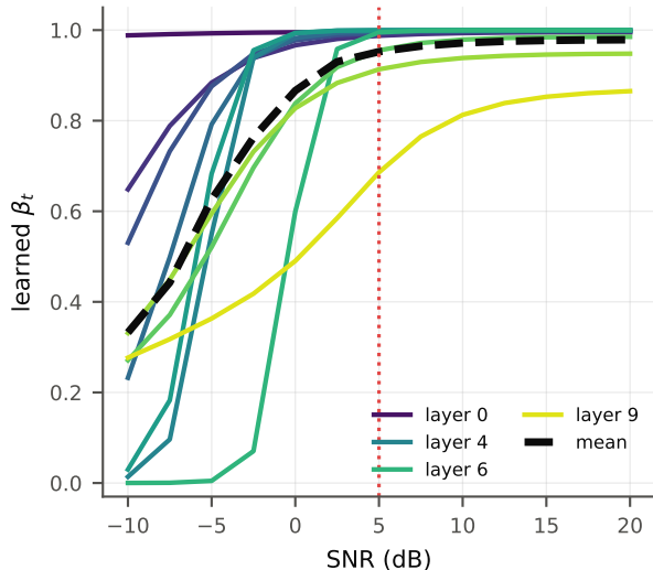
a. G2: \beta rises with SNR in every layer (mean 0.33 \rightarrow 0.98)
