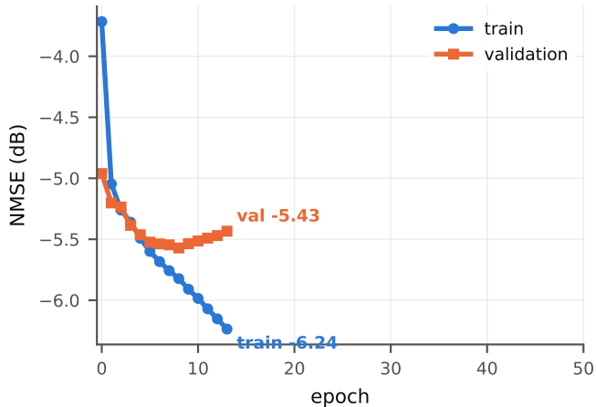
arm 1a — training, 14/50 epochs
