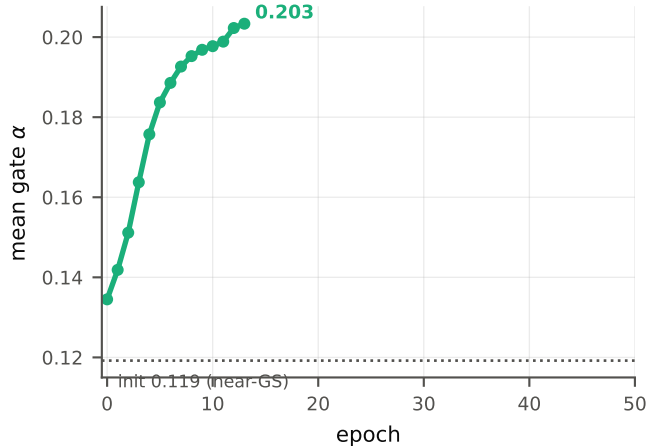
gate drifts toward EM-GS ( \alpha \rightarrow 1 )
