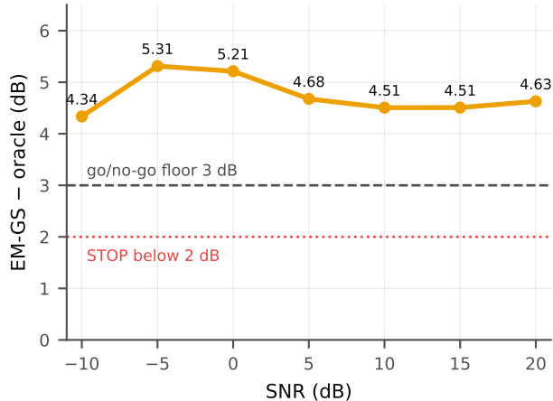
headroom: 4.34–5.31 dB, all points pass
