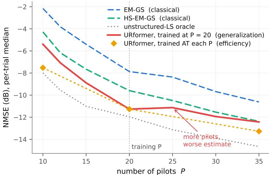
Pilot efficiency and pilot-count generalization are different curves SNR = 5 dB, 400 paired trials per point
