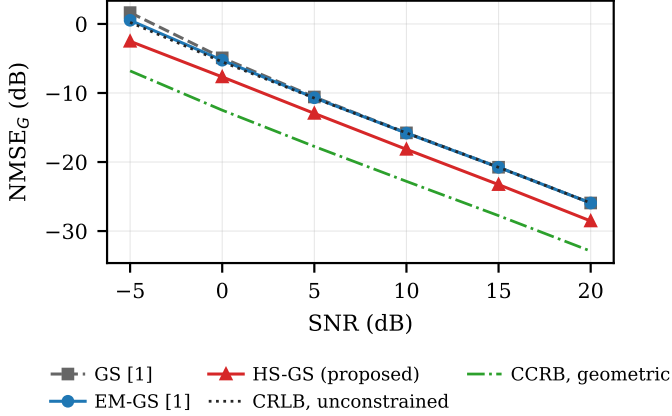
Fig. 1. NMSE versus SNR, bound-comparison configuration ( N = 32 , P = 30 , RSR 12 dB, T = 50 , 4 Cadzow sweeps, ratio-of-sums). EM-GS tracks the rank-one unconstrained CRLB to within 0.164 dB above 5 dB. Neither bound governs a biased estimator.
