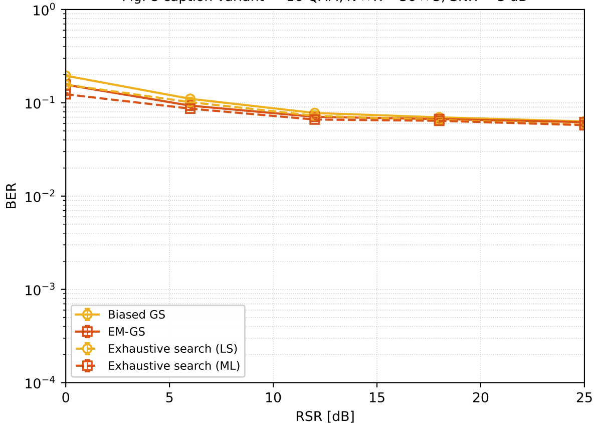
Fig. 8 caption variant — 16-QAM, N \times K = 36 \times 3 , SNR = 3 dB
