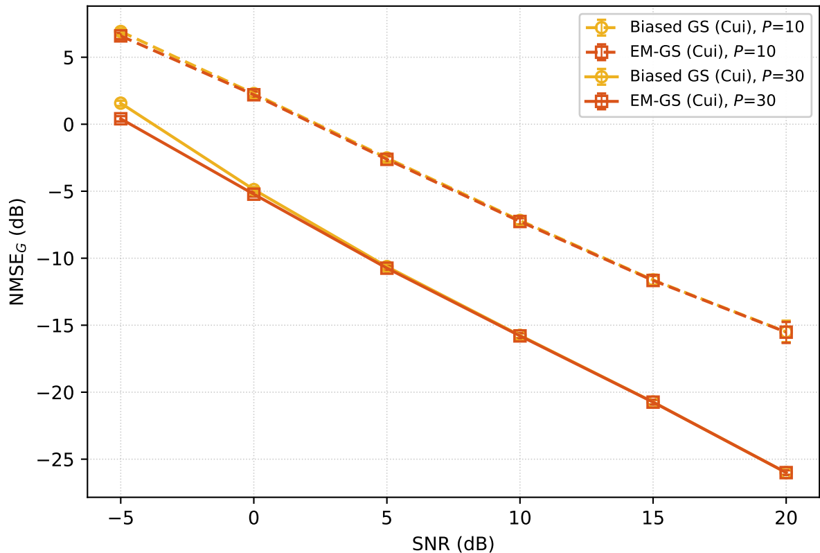
B1 — channel NMSE vs SNR N=8, K=3, L_k \sim \mathcal{U}\{3..7\}, \text{RSR}=12 \text{ dB}, t_0=50, 400 \text{ trials/point}
