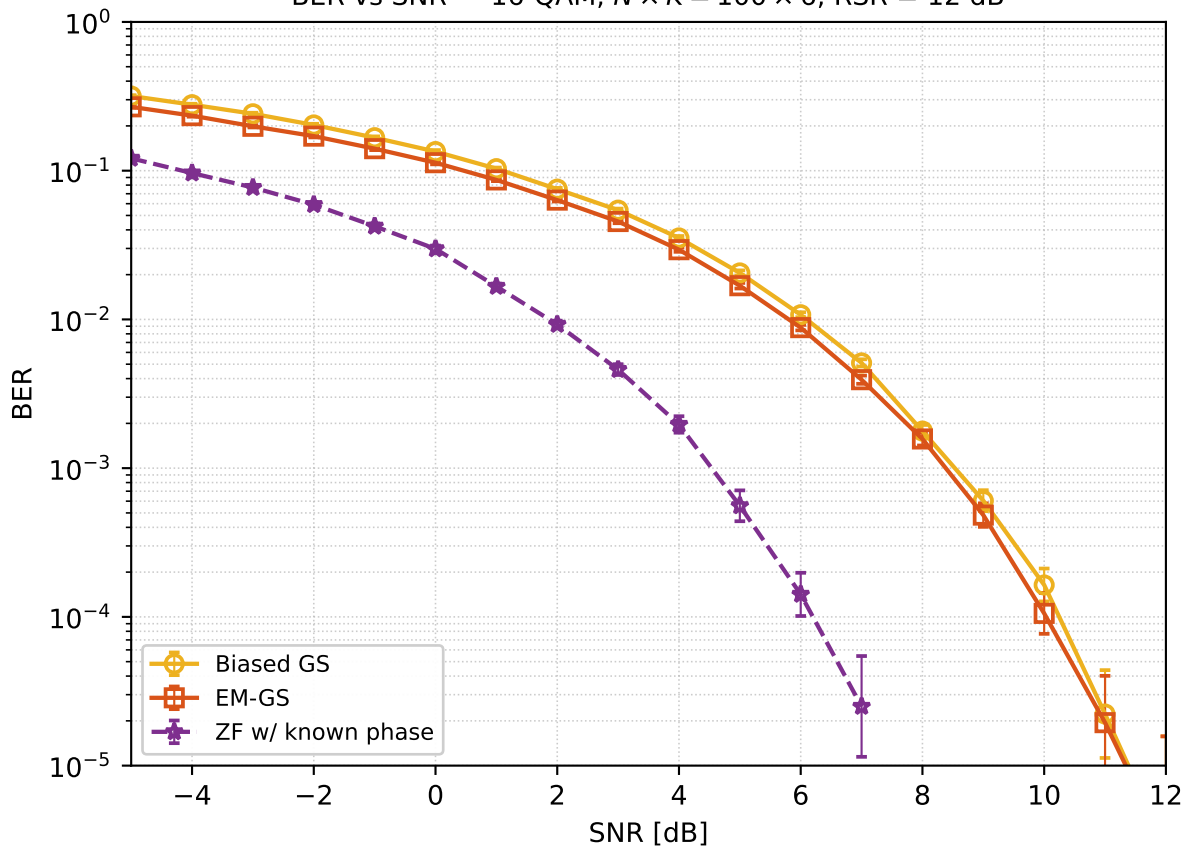
BER vs SNR — 16-QAM, N \times K = 100 \times 6 , RSR = 12 dB
