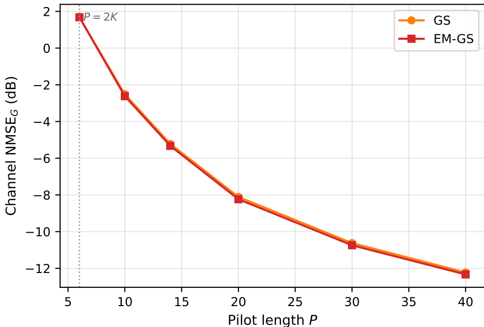
A2: baselines vs pilot length ( N=8 , SNR=5 dB)
